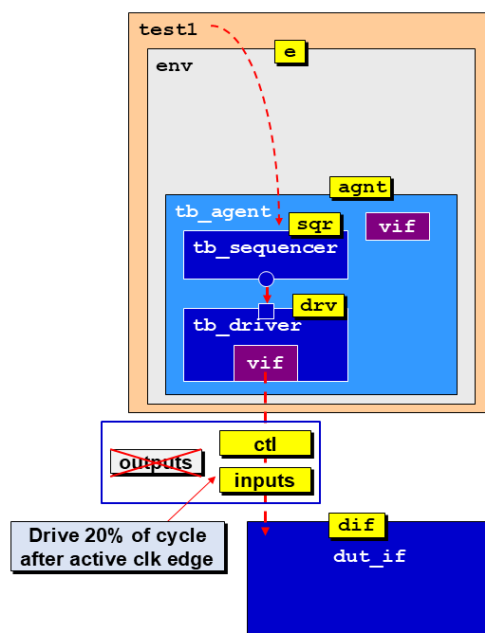
Figure 3 - Stimulus driving half of UVM testbench
